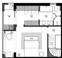
2F PLAN
